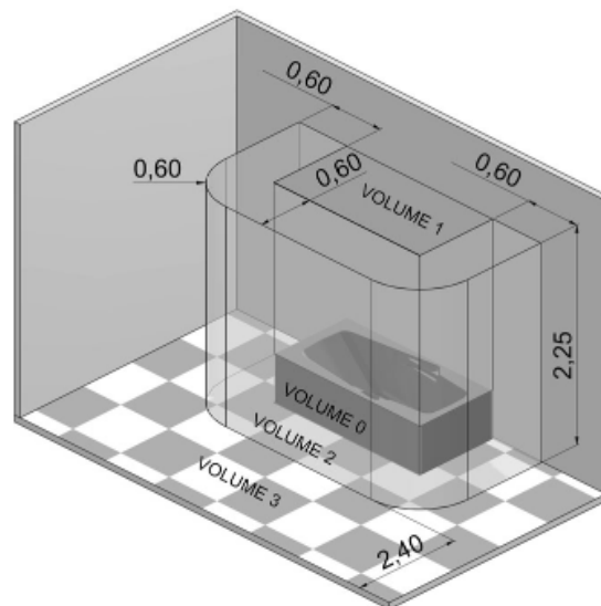
Authorised water heater fixing zones:
